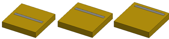
Fig. 5. Different positions of the graphene patch with respect to the substrate: patch in the center of the substrate (left), at 1.25 \mu\text{m} from the center (middle) and at 2.5 \mu\text{m} from the center (right).
