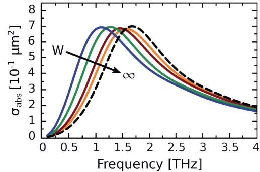
Fig. 3. Dependence of the absorption cross section of a graphenna as a function of its width. The absorption cross section normalized to the graphenna width is shown. The length of the graphenna is L = 5 \mu\text{m} . The plots correspond to infinite, 10 \mu\text{m} , 5 \mu\text{m} , 2 \mu\text{m} and 1 \mu\text{m} wide patches (right to left).
