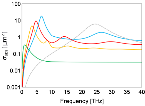
Fig. 8. Absorption cross section (in logarithmic scale) of a graphenna as a function of frequency, for different values of the chemical potential: 0 (green line), 0.5 (yellow line), 1 (red line) and 2 eV (blue line). The results are compared to that of an equivalent gold antenna with the same size (gray dashed line).
