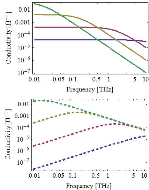
Fig. 9. Log-log plots of the real (above) and imaginary (below) parts of the electrical conductivity of graphene as a function of the frequency, for different values of the relaxation time: 10^{-14} s (blue line), 10^{-13} s (purple line), 10^{-12} s (yellow line) and 10^{-11} s (green line).
