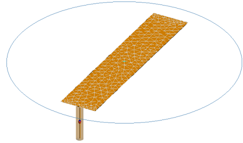
Fig. 11. Schematic diagram of the graphenna in transmission. The graphenna is composed of a graphene patch with a length L = 5 \mu\text{m} and a width W = 1 \mu\text{m} , and a pin feed located at 0.1 \mu\text{m} from the edge of the graphenna. The blue circle shows the plane in which the radiation diagram is measured.
